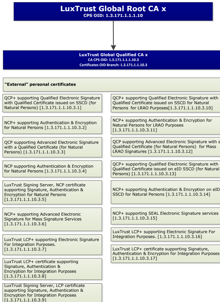
Figure 3 - LuxTrust Global Qualified CA Hierarchy
